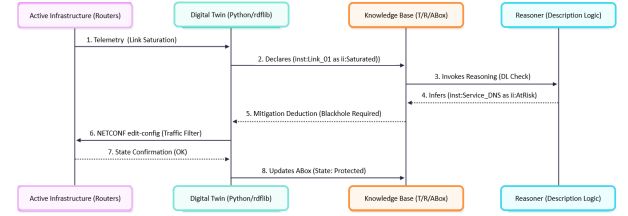
Fig. 3: Sequence Diagram of DDoS Mitigation via DT-II
